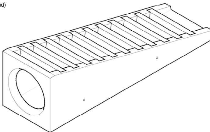
EMBOCADURA SALVACUNETA C-60 (HRF)*
